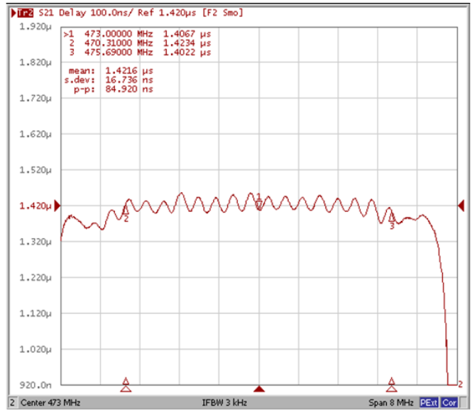
Group Delay Variation Fo±2.69MHz
