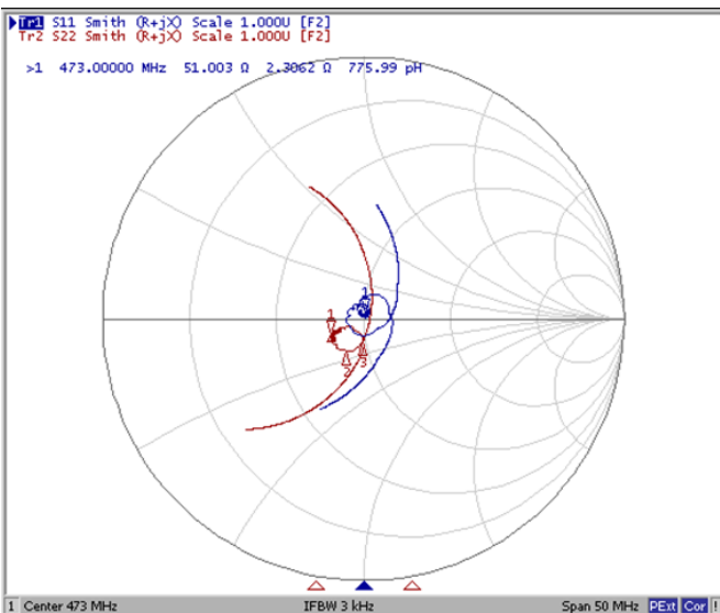
Smith Chart
